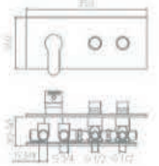
ARF5030T2 Concealed brass two function mixer Finish: Chrome
