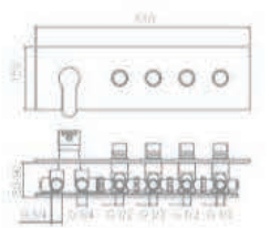
ARF5030T4 Concealed brass four function mixer Finish: Chrome
