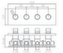
ARF5034T2 Concealed brass two function mixer Finish: Chrome
