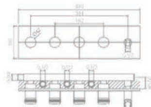
ARF5052T4+1 Concealed brass four function mixer Finish: Chrome
